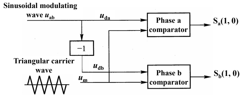
Figure 3. Diagram of unipolar SPWM for the two-level PWM rectifier.
